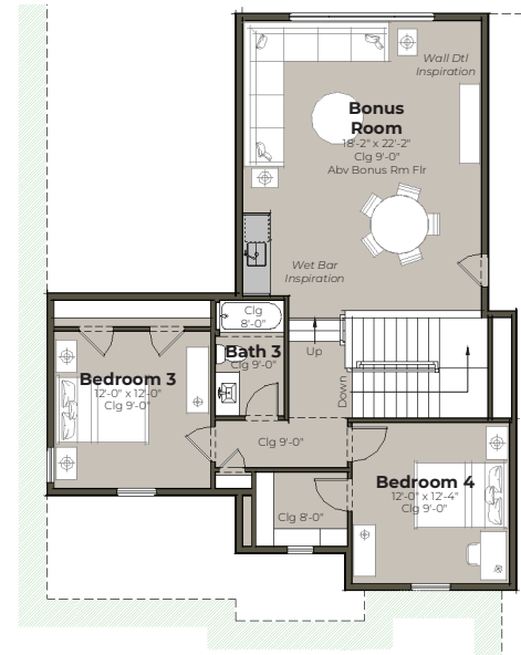
Second Floor I
