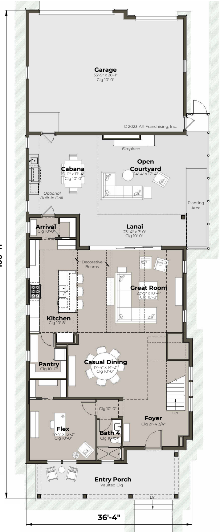
First Floor
