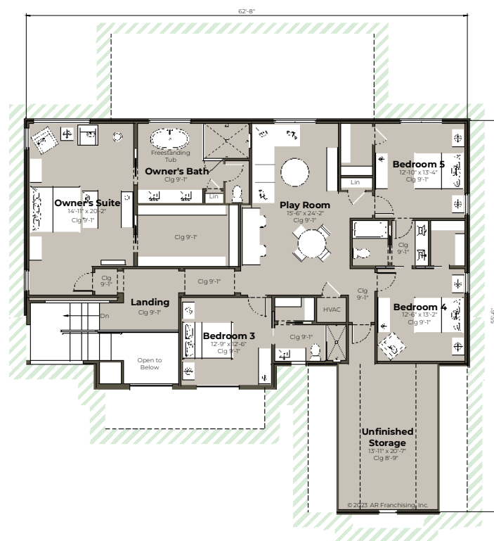
Second Floor
