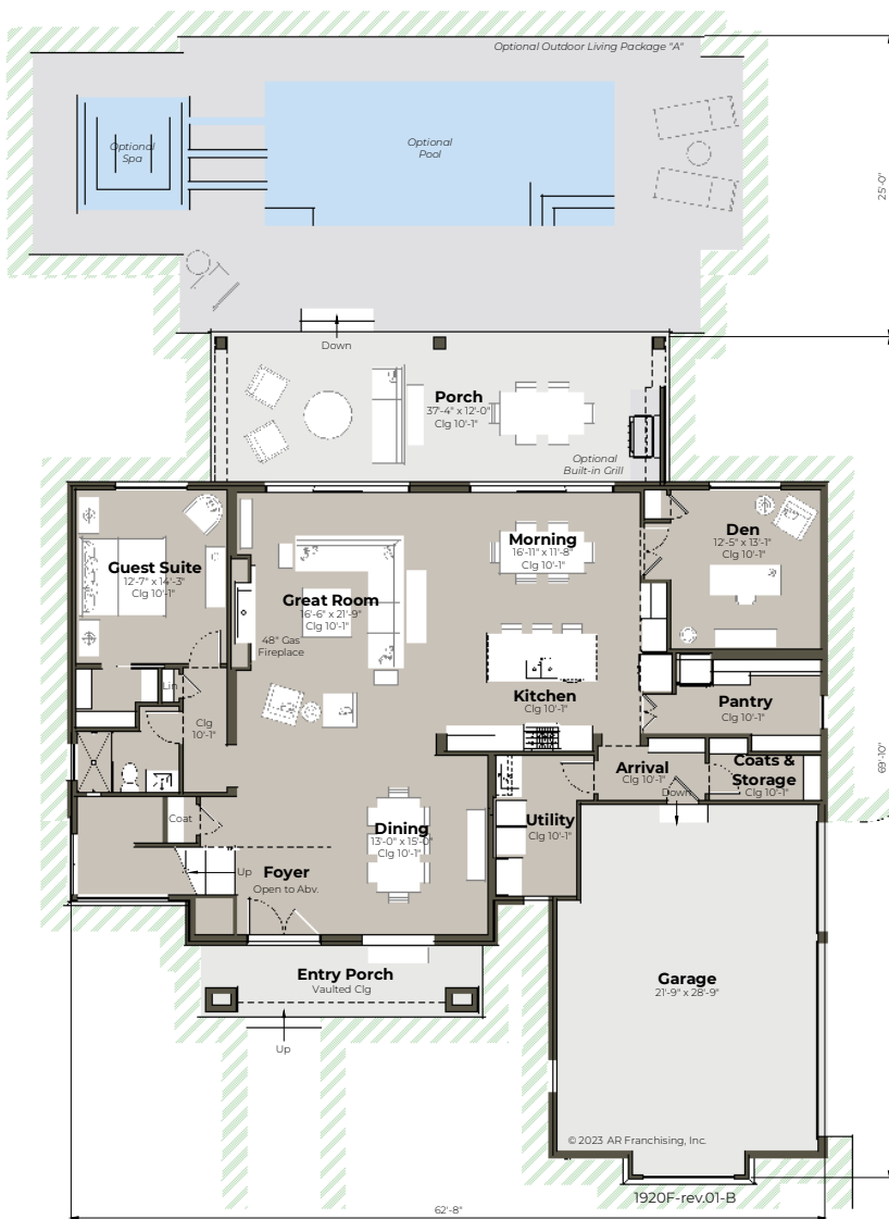
First Floor
