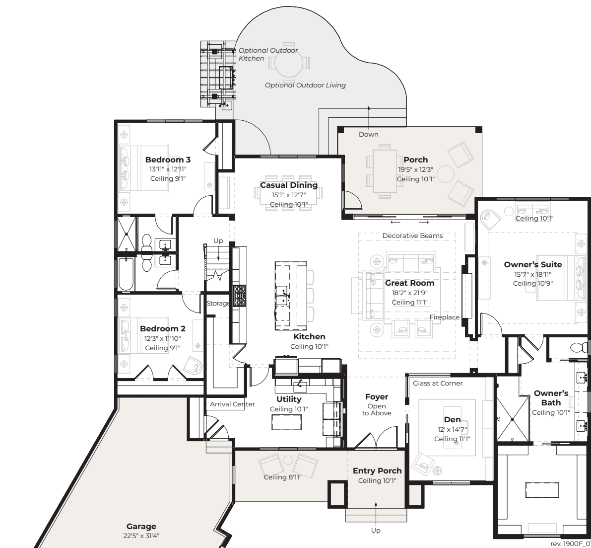
First Floor
