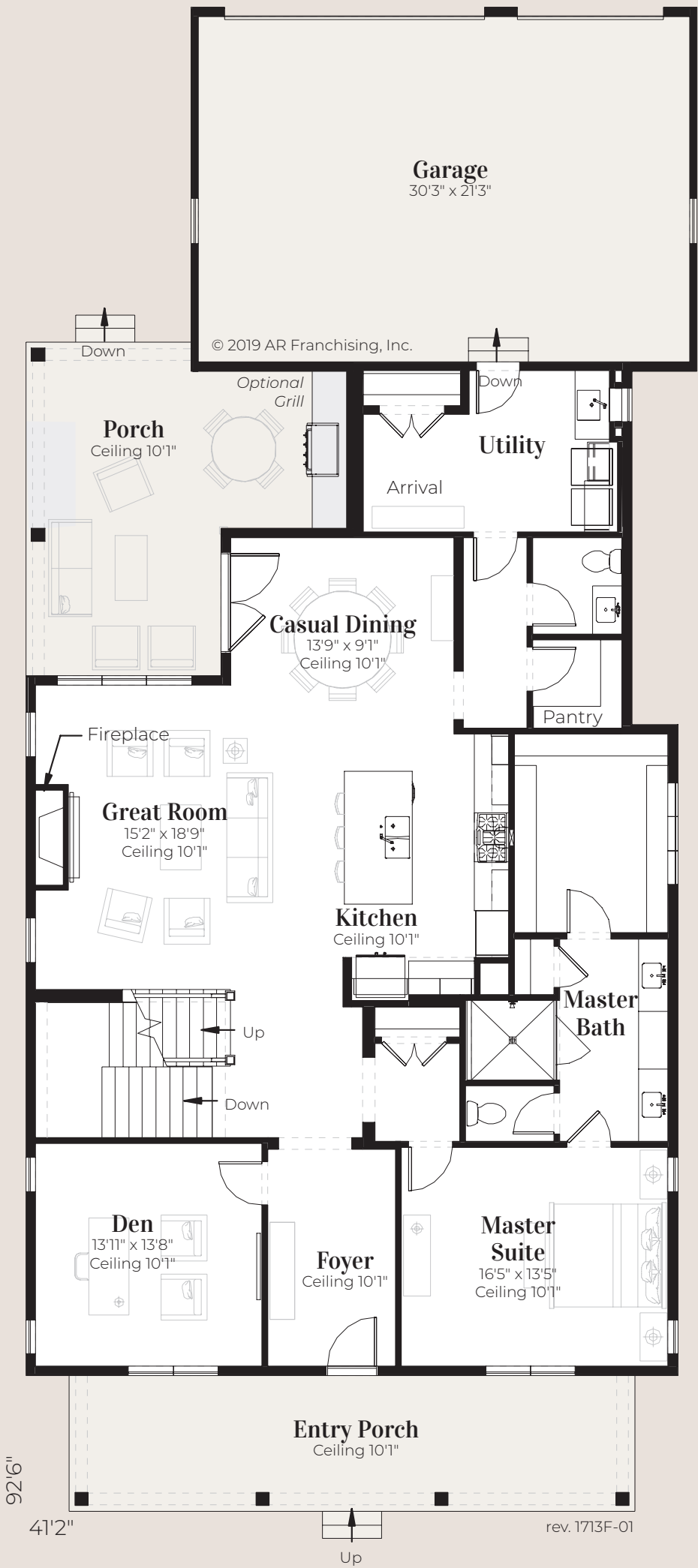
Main Level
