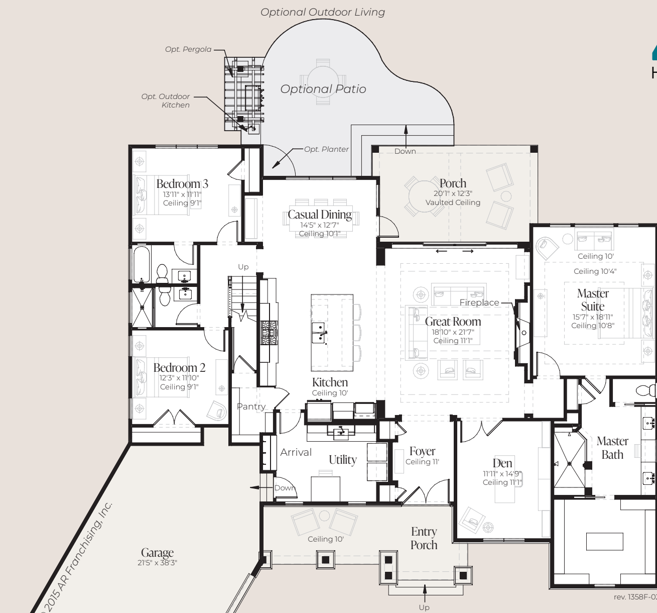
Main Level
