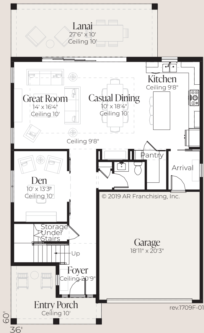
Main Level
